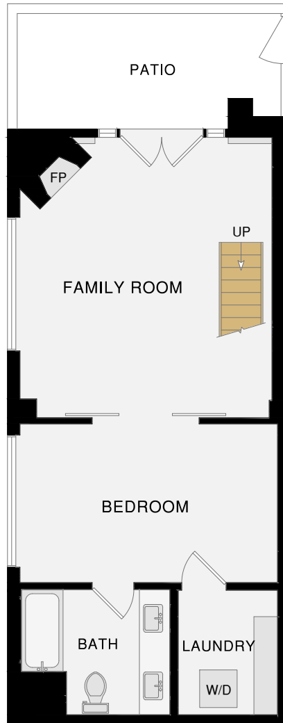
LOWER LEVEL
